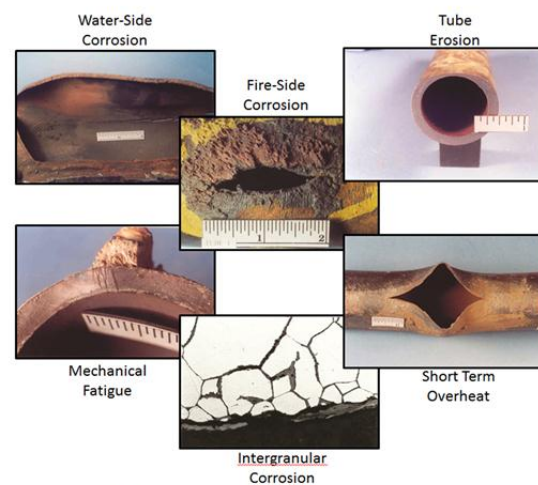
Figure 2. Metallurgical samples representing several significant failure mechanisms affecting tubing in the utility industry. Identifying the root cause of the failure, as seen above, is paramount to comprehensively reducing future forced outages.]
