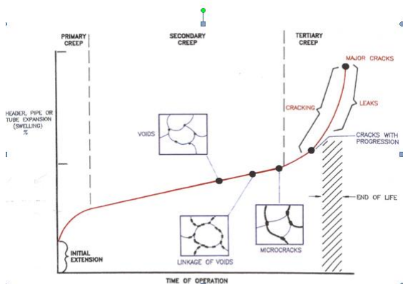
Figure 4. Stages of Creep Development. As creep stages progress, illustrated in the graphic above, the voids begin to link with one another, developing into cracks which then propagate through the material eventually causing leaks or failures.
